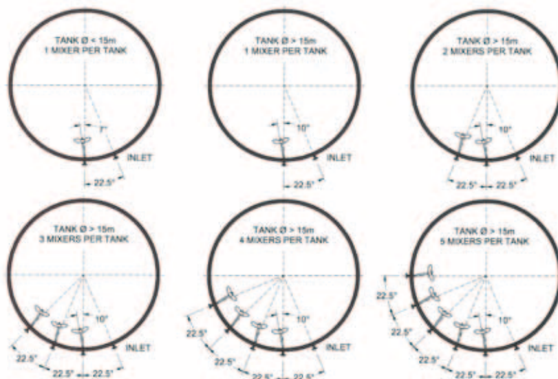
Plenty recommended mixer (Fixed Angle) positions for effective blending, homogeneity and temperature uniformity
